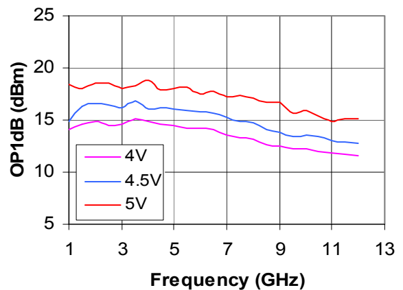
Figure 12. Output P1dB Over Vdd
