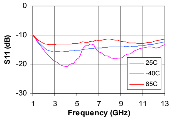
Figure 17. Input Return Loss Over Temp
