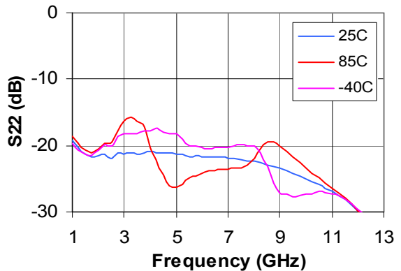
Figure 18. Output Return Loss Over Temp
