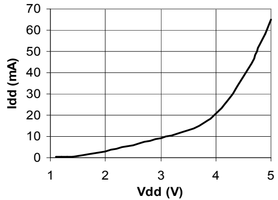
Figure 8. Total Current
