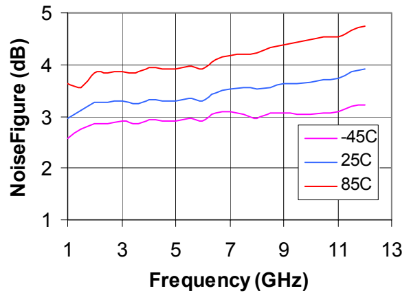
Figure 16 Noise Figure over Temp
