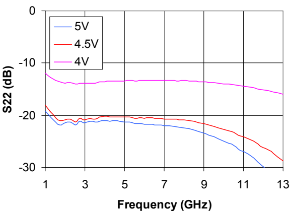
Figure 11. Output Return Loss Over Vdd
