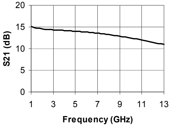
Figure 1. Small-signal Gain
