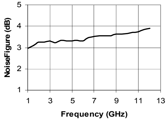
Figure 2. Noise Figure
