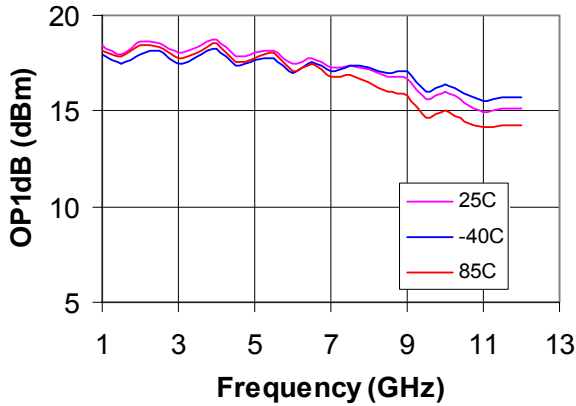
Figure 13. Output P1dB over Temp
