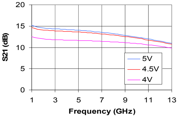
Figure 7. Gain over Vdd
