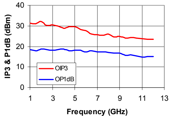
Figure 6. Output IP3
