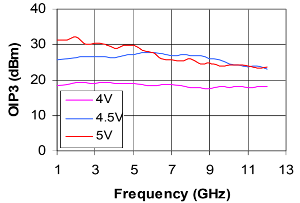
Figure 14. Output IP3 over Vdd
