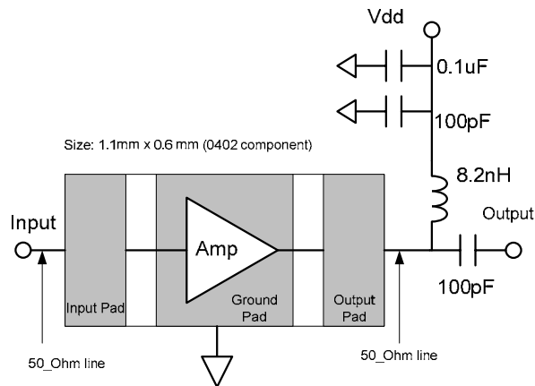
Figure 20. Evaluation/Test Board (available to qualified customer request)
