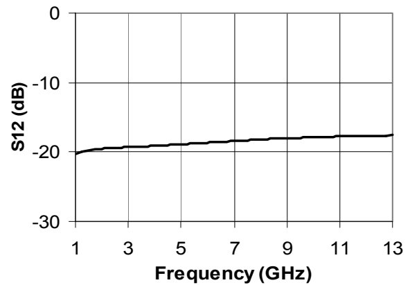
Figure 4. Isolation
