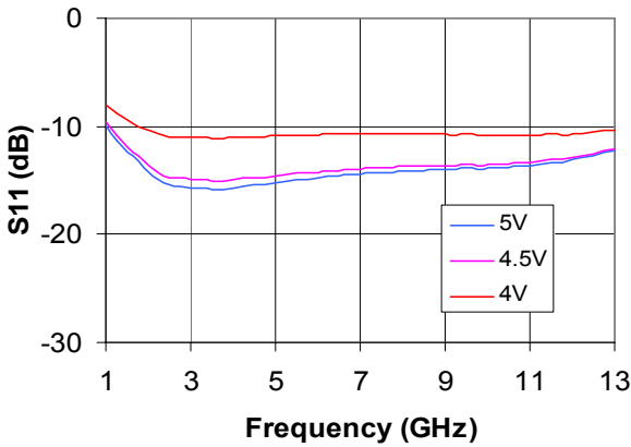
Figure 9. Input Return Loss over Vdd
