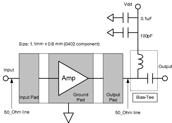
Figure 19. Usage of the VMMK-2503
